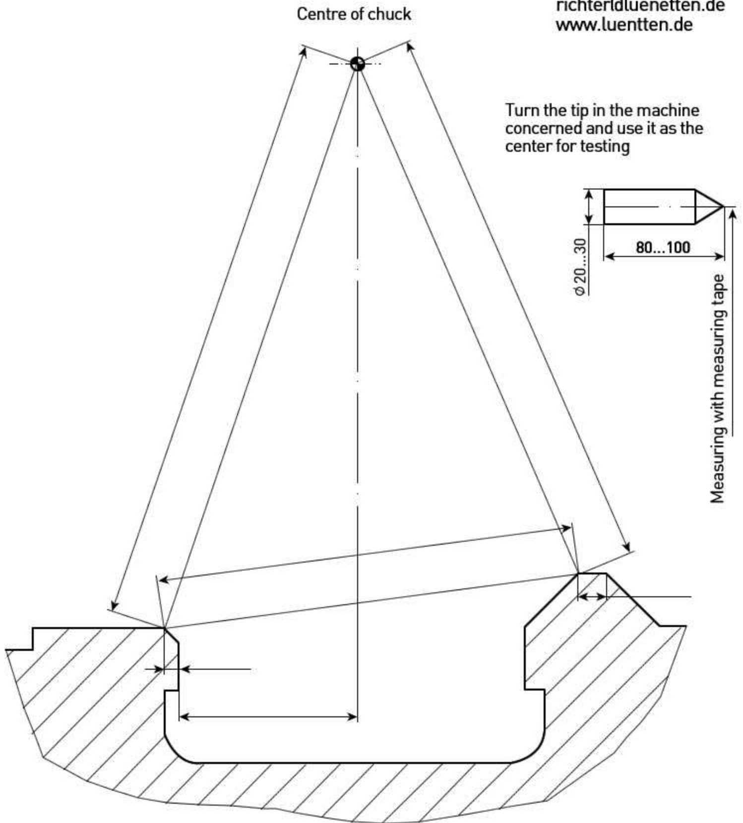
Dimension sheet for determination of pitch
